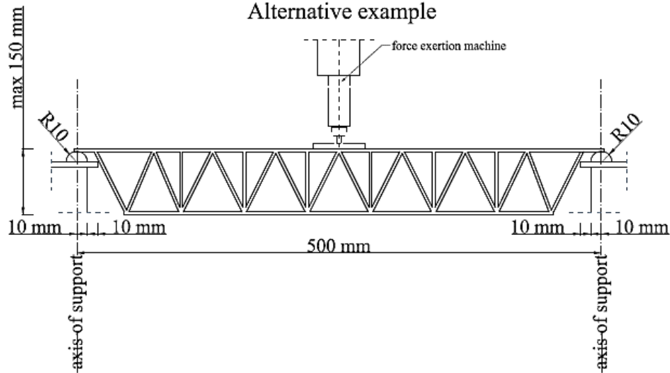
Picture ٧. The loading scheme of an exemplary model.
