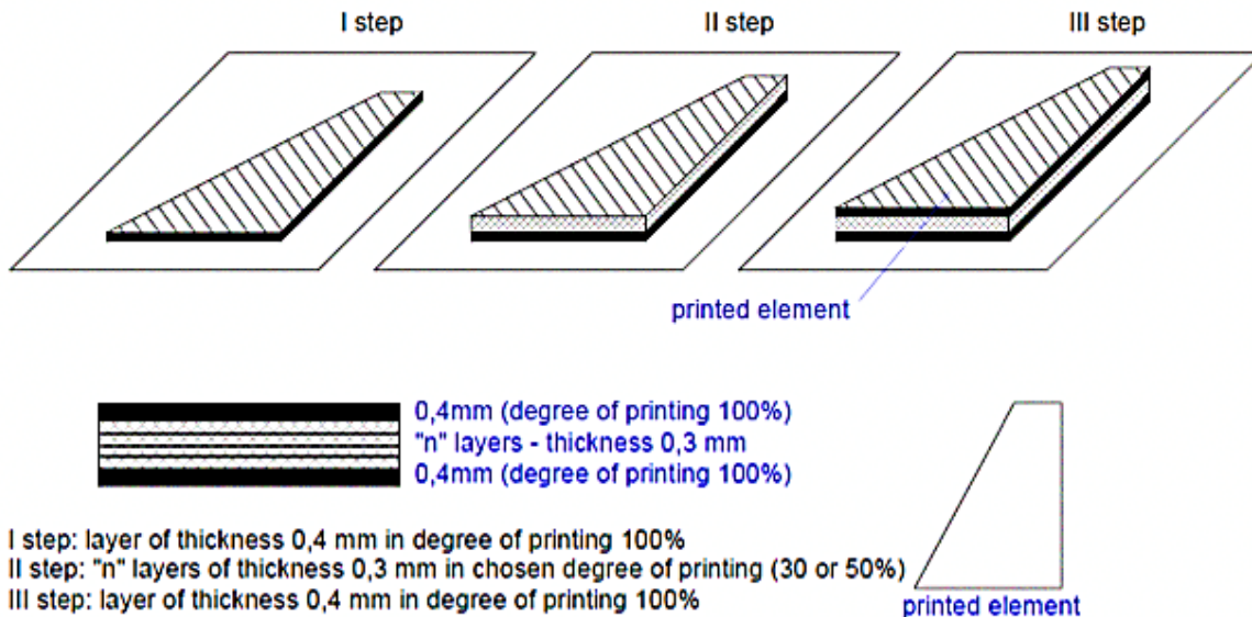
Picture ٧. Steps of printing an element on the 3D printer.
