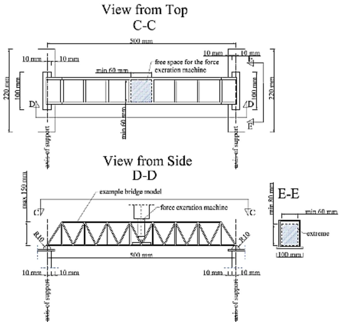
Picture ٧. The loading scheme of an exemplar model with marked required extremes.
